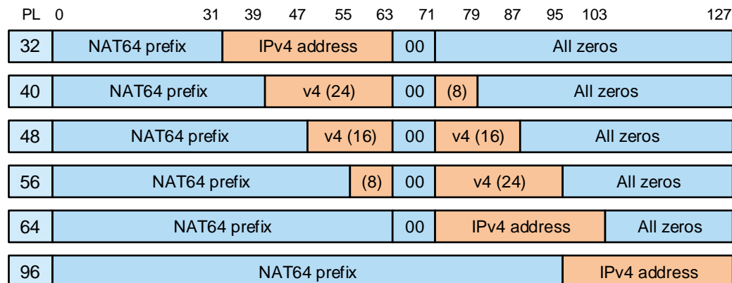
Figure 5-1 IPv6 Address Formats for Different NAT64 Prefix Lengths
